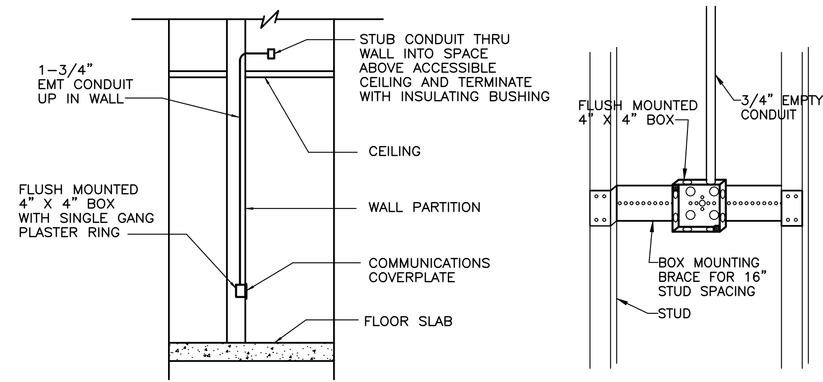
1 COMMUNICATIONS OUTLET WALL INSTALLATION NTS
