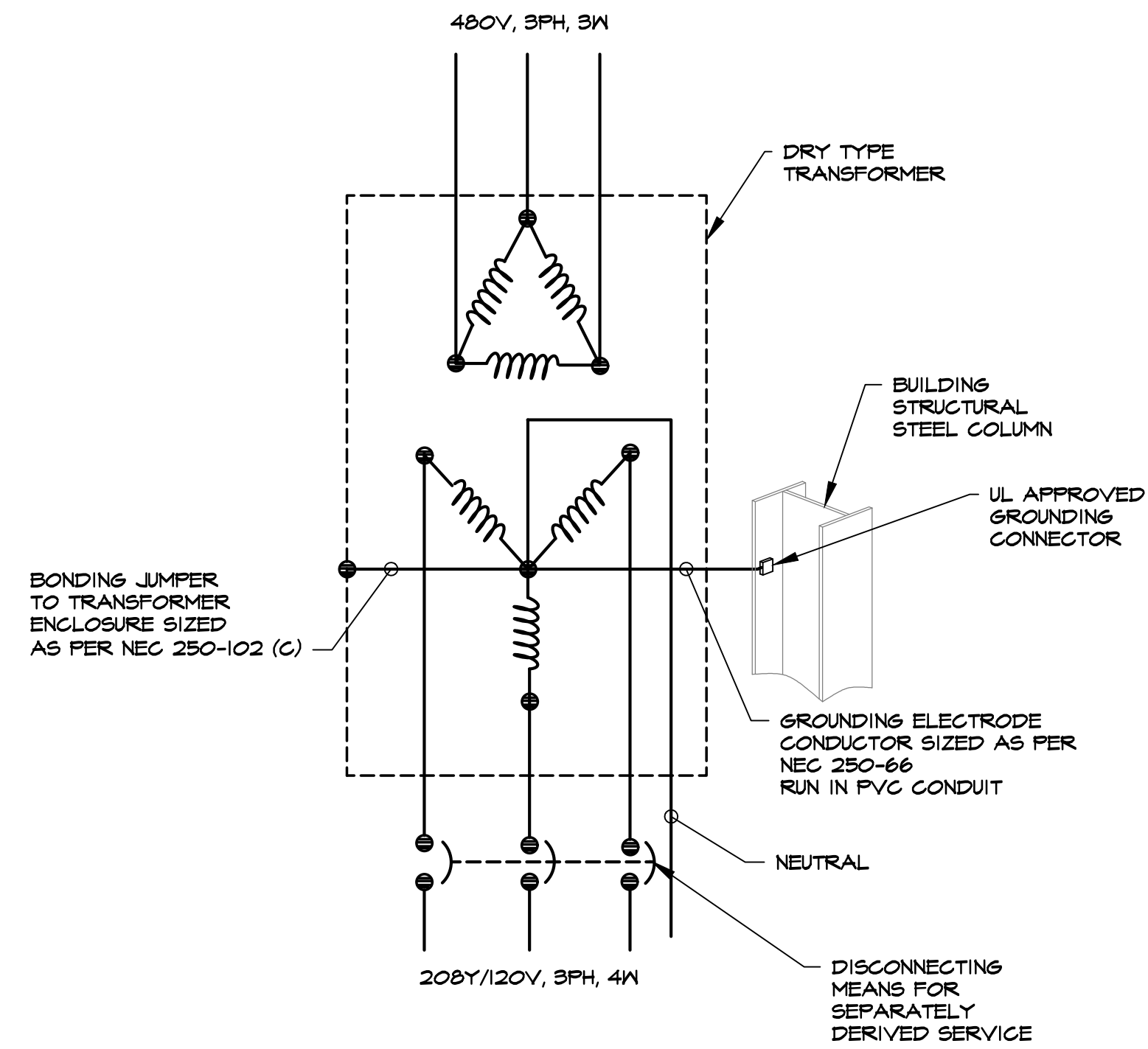
2 TYPICAL GROUNDING PROCEDURE FOR 3-PHASE DRY TYPE TRANSFORMER INSTALLATIONS NTS
