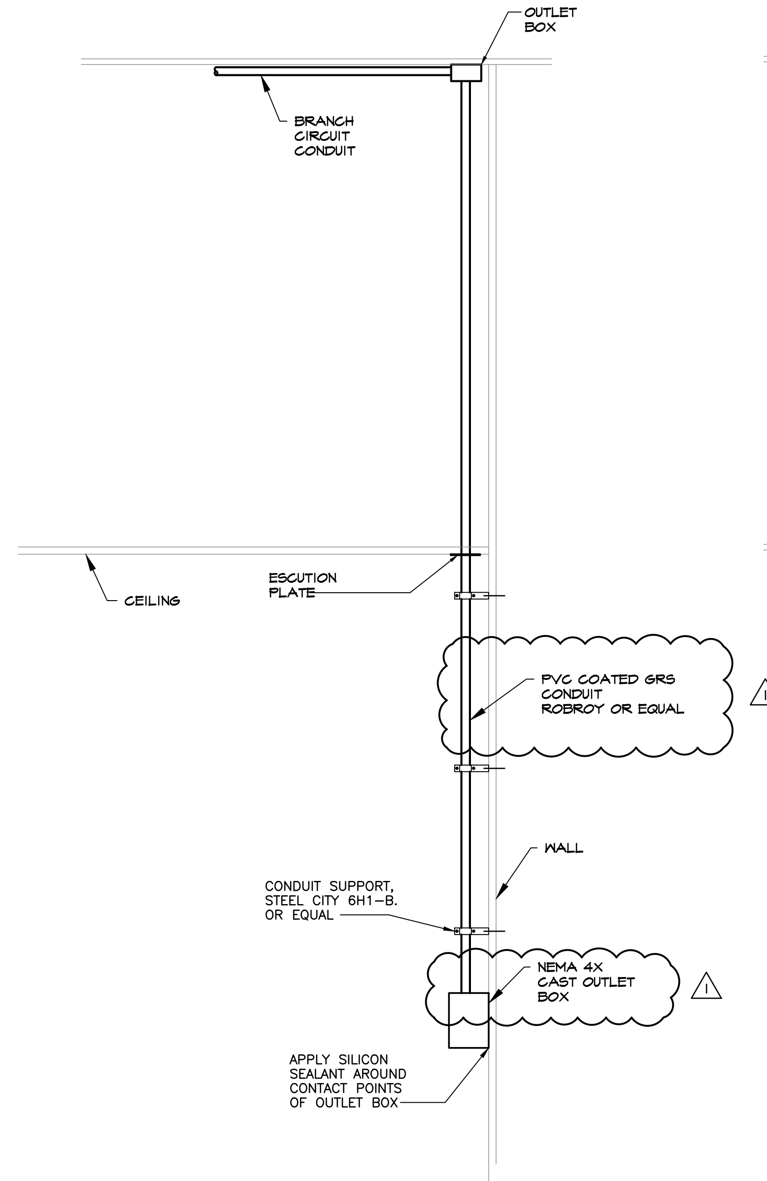
3 EXPOSED CONDUIT INSTALLATION DETAIL AT FOOD PROCESSING AREAS NTS
