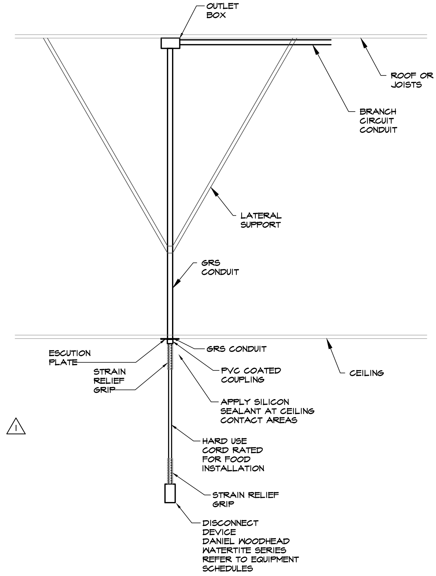
4 DISCONNECT INSTALLATION DETAIL AT FOOD PREP LINES NTS
