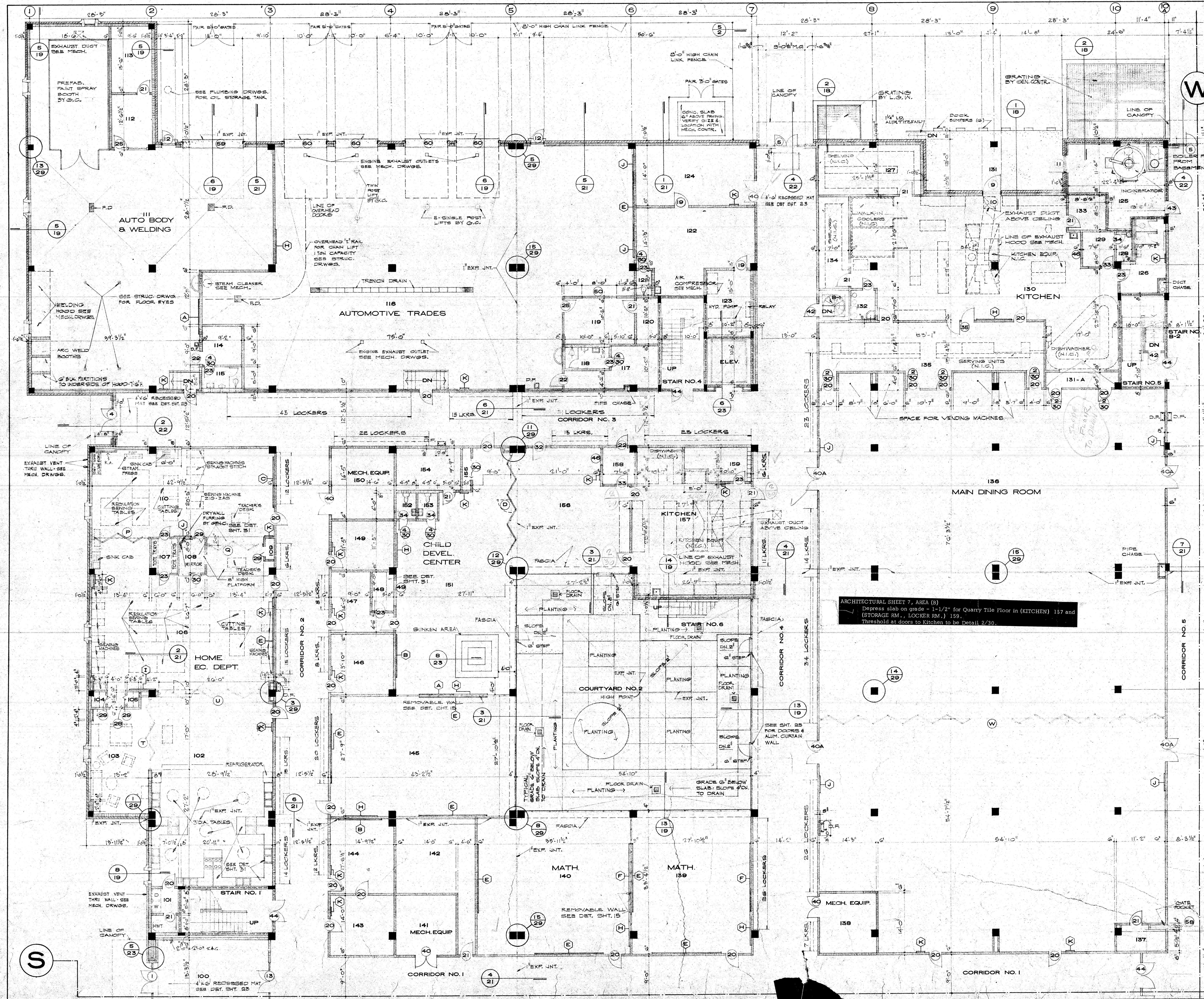
FIRST FLOOR - AREA (B) SCALE 1/8" = 1'-0"
