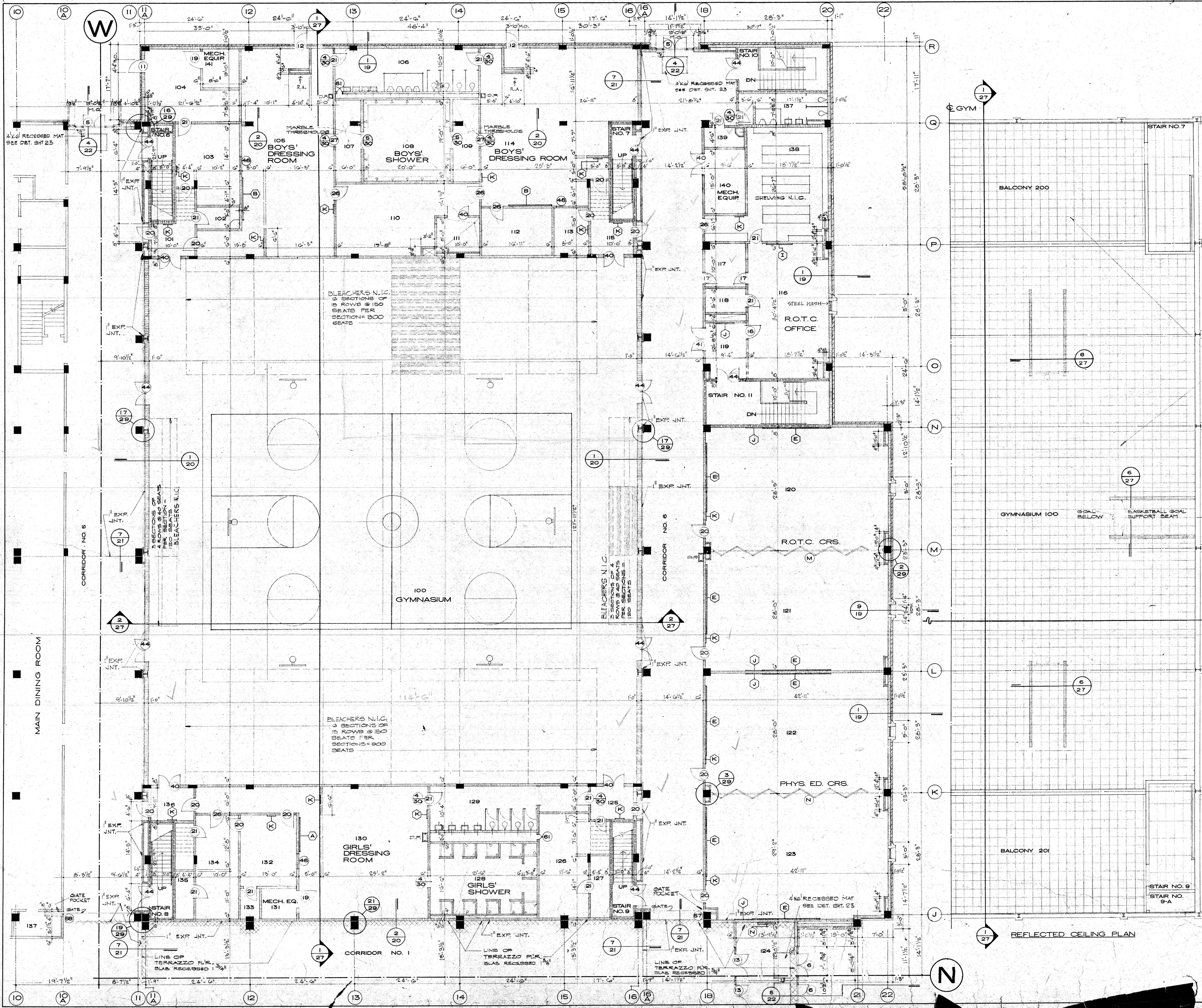
FIRST FLOOR - AREA C SCALE: 1/8" = 1'-0"
