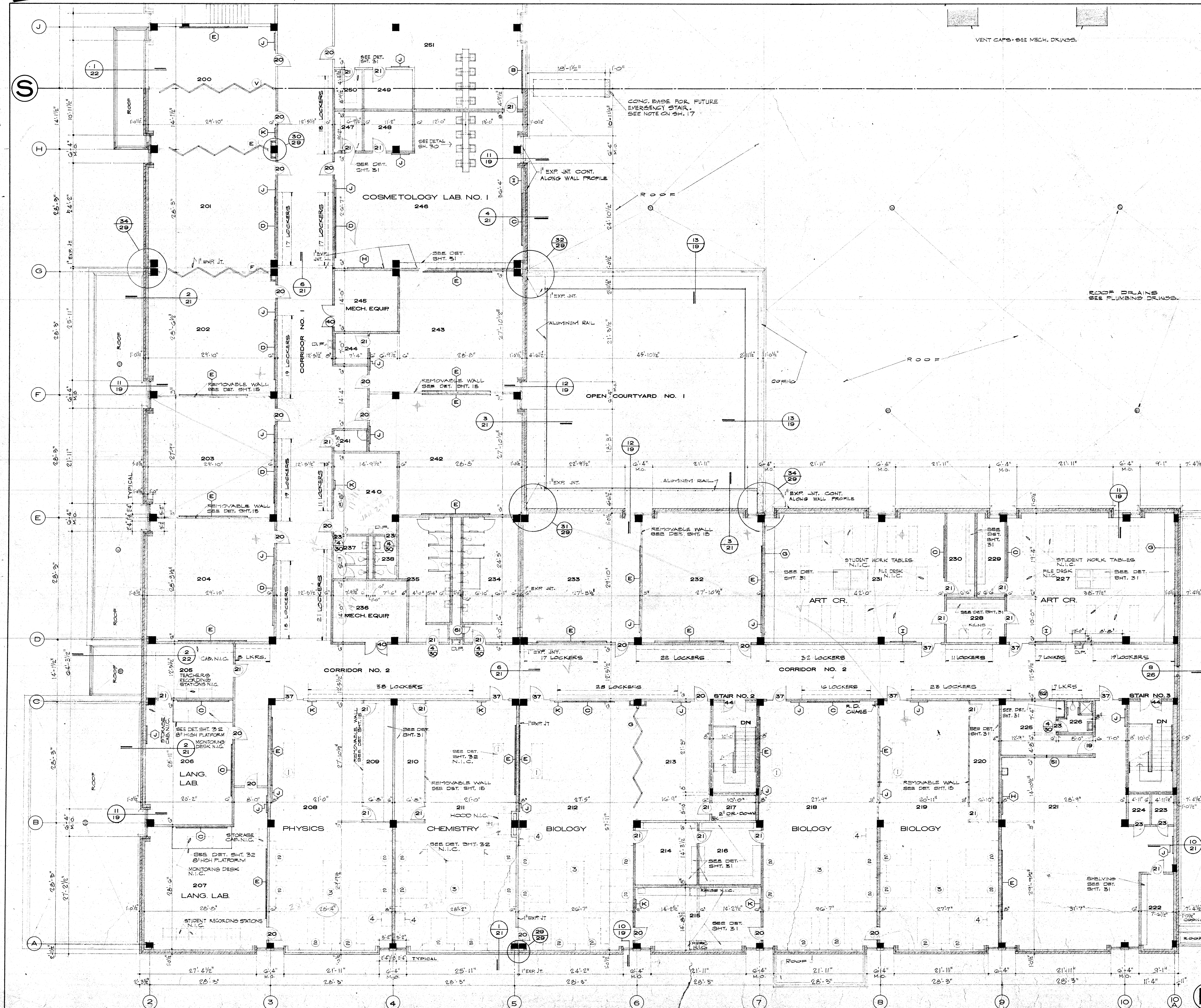
SECOND FLOOR - AREA E SCALE 1/8" = 1'-0"
