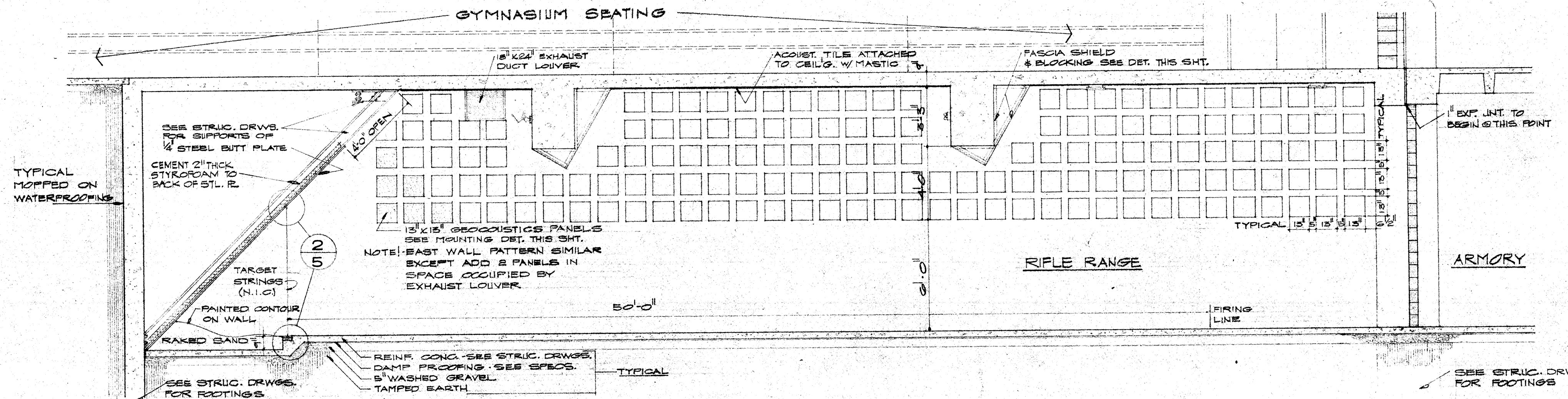
1/5 CROSS SECTION R.O.T.C. RIFLE RANGE SCALE: 1/4" = 1'-0"
