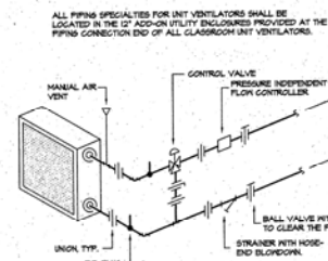
WATER COIL PIPING SCHEMATIC
