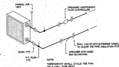
HOT WATER UNIT HEATER PIPING SCHEMATIC
