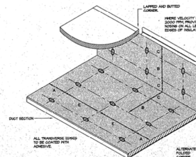
INTERNAL DUCTLINER DETAIL
