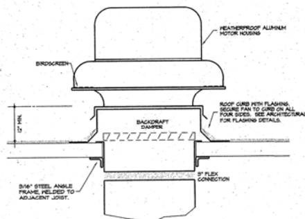
ROOF MOUNTED EXHAUST FAN DETAIL
