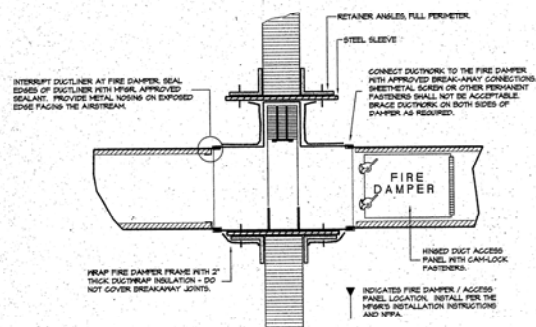
VERTICAL FIRE DAMPER DETAIL
